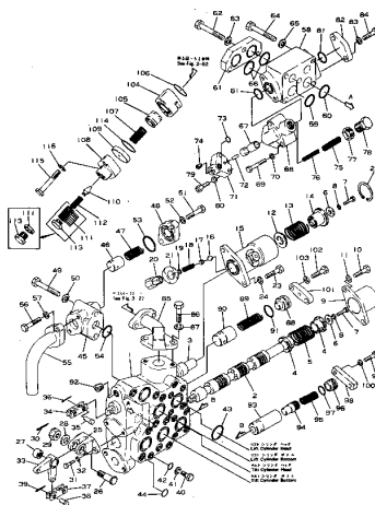
Fig. 104 HYDRAULIC CONTROL VALVE DDC050-1A,1C / 適用号機 DDR050-1A,1B (Serial No. 1001 ~)
