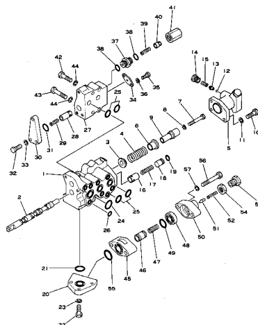
Fig. 135 HYDRAULIC CONTROL VALVE (1/2)
