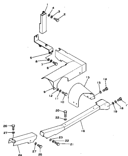
Fig. 122 HYDRAULIC OIL PIPING COVER
