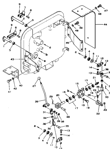
Fig. 132 HYDRAULIC TANK (2/2)
