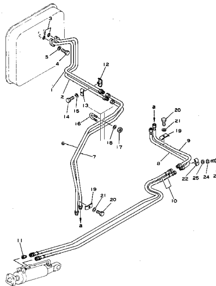
Fig. 121 HYDRAULIC OIL PIPING
