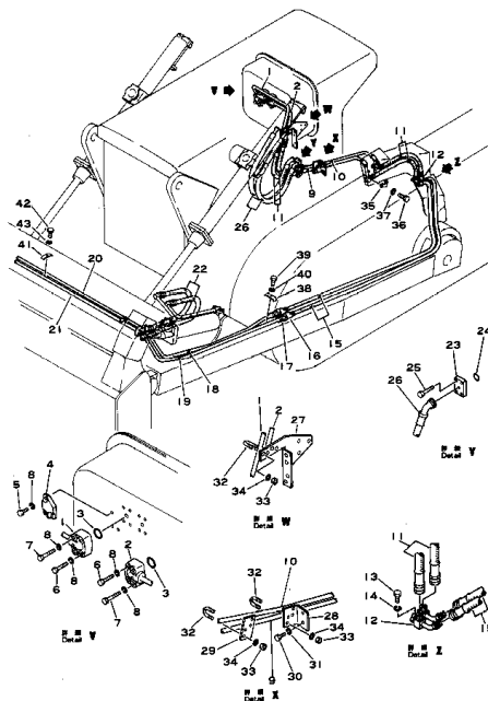
Fig. 121A HYDRAULIC PIPING (Serial No. (1801)~)
