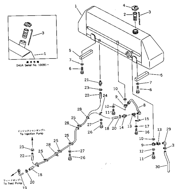
FIG. 1303 FUEL TANK AND PIPING (FOR TRIMMING DOZER) 適用機種 (D41A SERIAL NO. 10001-)
