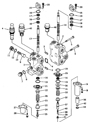
Fig. 135 HYDRAULIC CONTROL VALVE (1/2)
