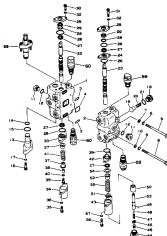
Fig. 121 HYDRAULIC CONTROL VALVE (1/2)
