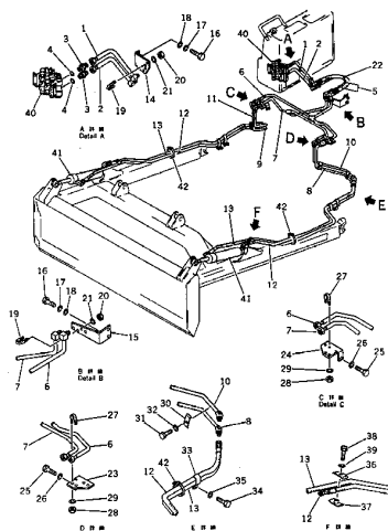
Fig. 221 HYDRAULIC OIL PIPING (適用機種: 2001~(50000))
