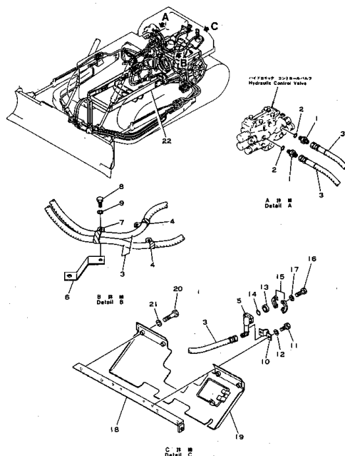
FIG. 121 HYDRAULIC PIPING (1/5)
