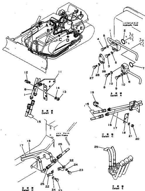
FIG. 123 HYDRAULIC PIPING (3/5)
