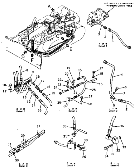
FIG. 124 HYDRAULIC PIPING (4/5) (適用機種 (Serial No.(1801-3305))
