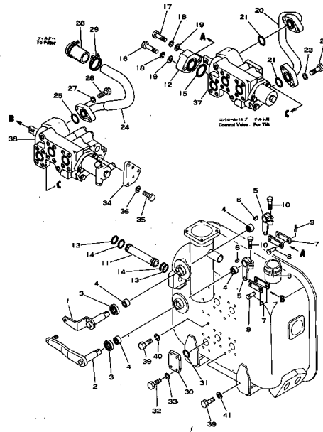
Fig. 122 HYDRAULIC TANK (2/2)
