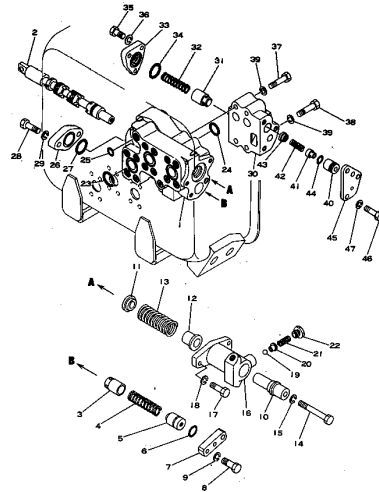
Fig. 125 HYDRAULIC CONTROL VALVE (1/2)
