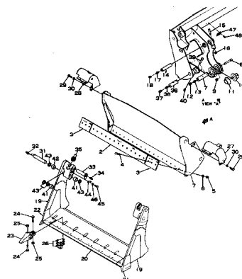
Fig. Fig01 BUCKET
