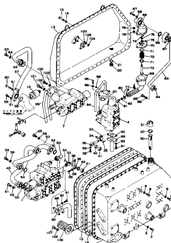
Fig. 103 HYDRAULIC TANK 1/2
