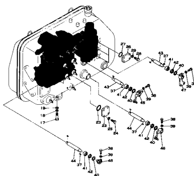
Fig. 103A HYDRAULIC TANK 2/2
