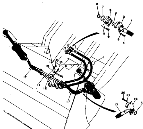
Fig. 103 HYDRAULIC PIPING (BUCKET SIDE) (Serial No. (1190~5021))
