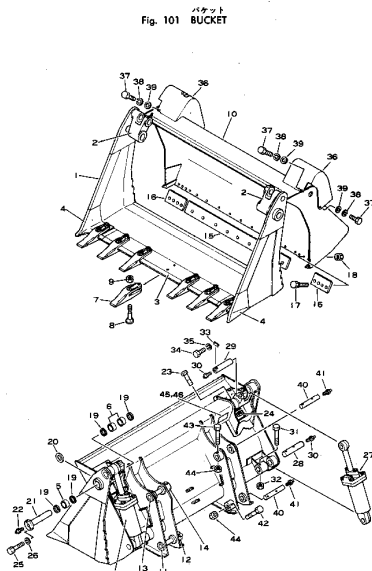
Fig. 101 BUCKET
