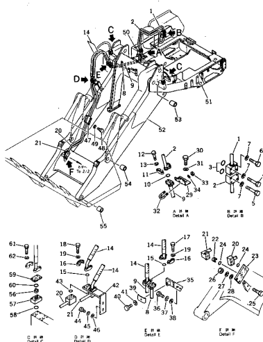
Fig. 121A HYDRAULIC PIPING (1/2) (DBM057-1A Serial No. (9001)~)
