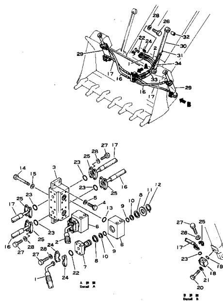
Fig. 125 HYDRAULIC PIPING (3/2)
