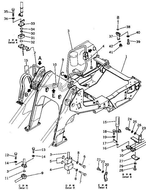
Fig. 121 HYDRAULIC PIPING (1/3)
