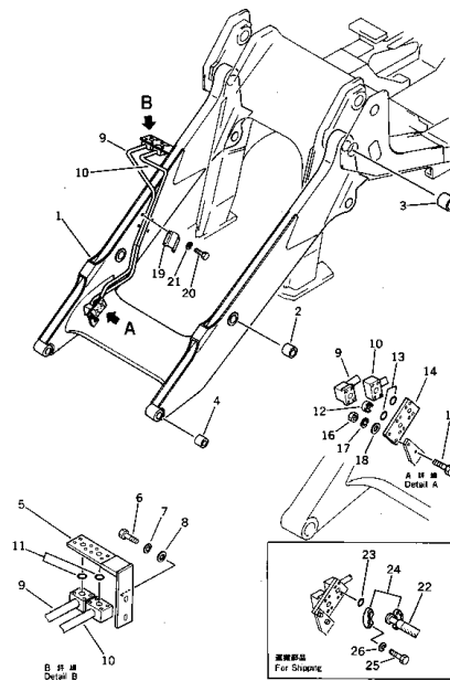
Fig. 122 HYDRAULIC PIPING (2/3)
