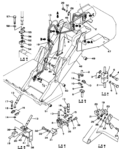
Fig. 121 HYDRAULIC PIPING (1/2) (DBM050-1A Serial No. 1001~) (DBM057-1A Serial No. 1001~(9000))
