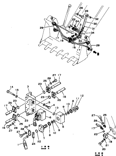
Fig. 125 HYDRAULIC PIPING (2/2)
