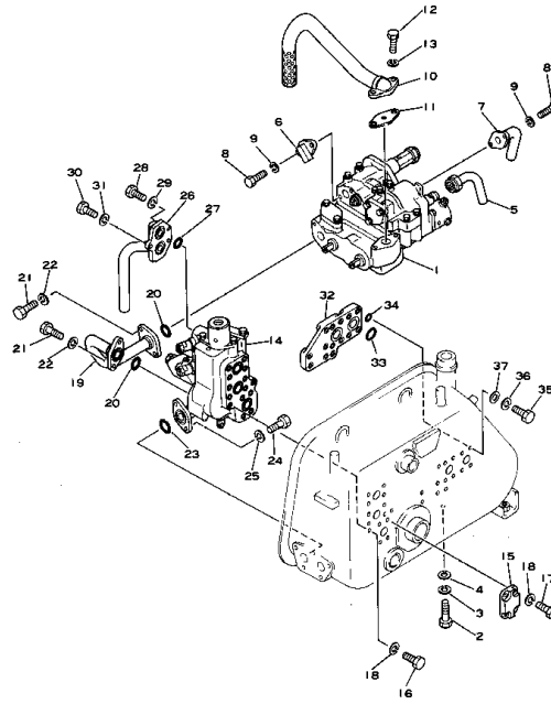
Fig. 132 HYDRAULIC TANK (2/3) (DBM050-1A Serial No. 1001~) (DBM057-1A Serial No. 1001~(9000))
