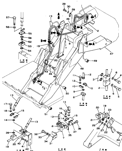
Fig. 121 HYDRAULIC PIPING (1/2) (DBD050-2C Serial No. 1001- ) (DBD050-2D Serial No. 1001- ) (DBD057-1A Serial No. 1001- (9000) ) (DBD057-1B Serial No. 1001- (9000) )
