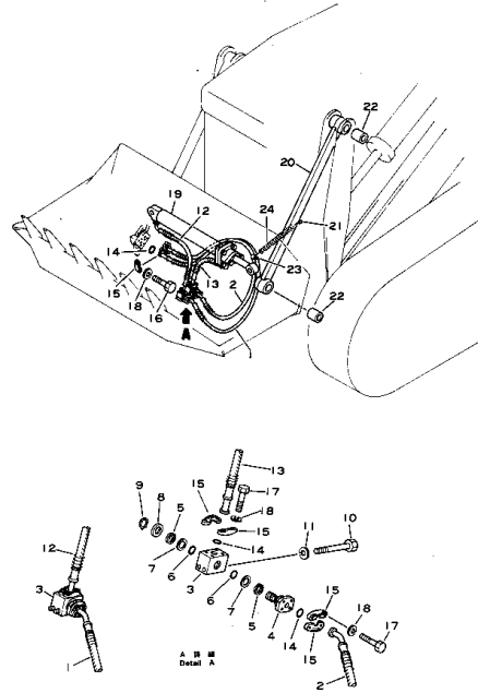
Fig. 125 HYDRAULIC PIPING (2/2) (DBD050-2C Serial No. 1001~ (DBD057-1A Serial No. 1001~(9000))
