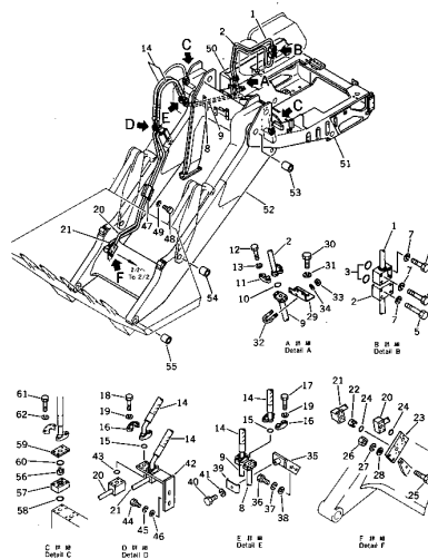
Fig. 121A HYDRAULIC PIPING (1/2) (DBD057-1A Serial No. (9001)~) (DBD057-1B Serial No. (9001)~)
