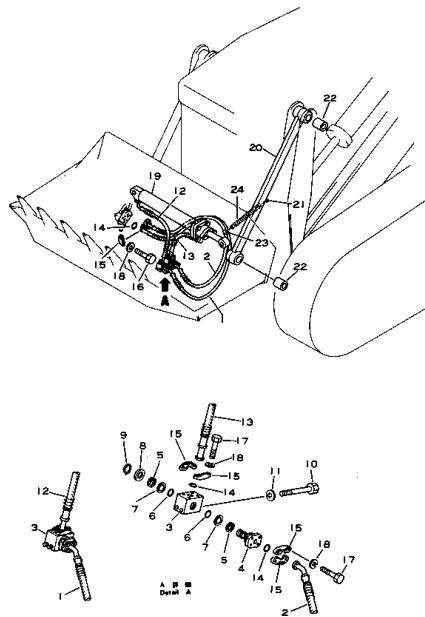
Fig. 125 HYDRAULIC PIPING (3/3) (DBD053-1A)
