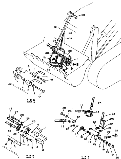
Fig. 126 HYDRAULIC PIPING (3/3) (DBD053-1B)
