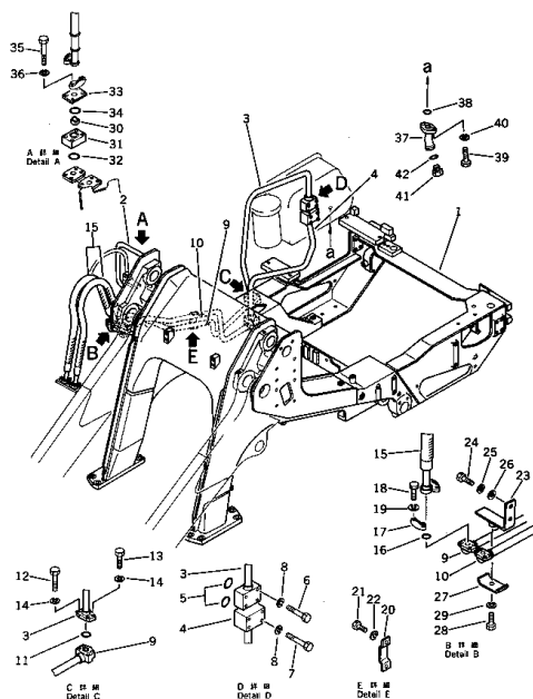
Fig. 121 HYDRAULIC PIPING (1/3)
