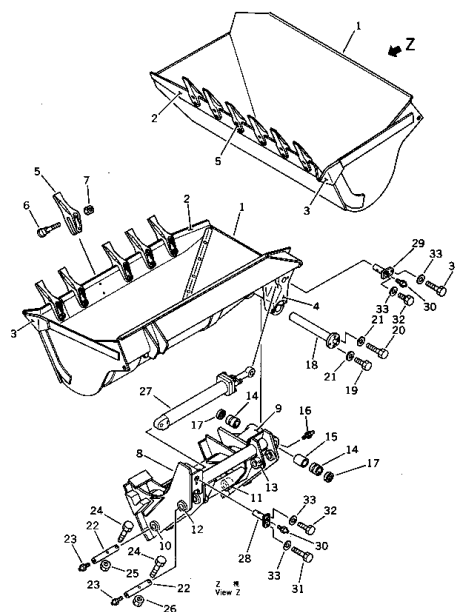
Fig. 102 BUCKET AND SUPPORT (DBD053-1B)
