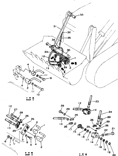
Fig. 126 HYDRAULIC PIPING (2/2) (DBD050-2D)
