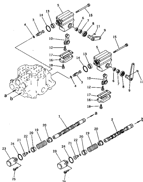
Fig. 136 HYDRAULIC CONTROL VALVE (%)
