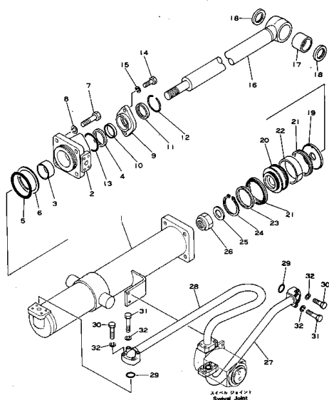
Fig. 111 CYLINDER (DBB050-1A Serial No. 1001~ (DBB057-1A Serial No. 1001~(9000))
