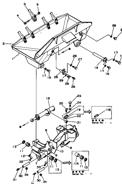
Fig. 101 BUCKET AND SUPPORT
