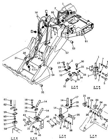
Fig. 121A HYDRAULIC PIPING (1/2) (DBB057-1A Serial No. (9001)-)
