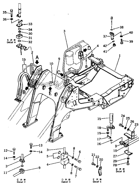
Fig. 121 HYDRAULIC PIPING (1/3)
