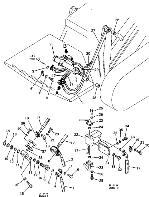
Fig. 125 HYDRAULIC PIPING (3/4)
