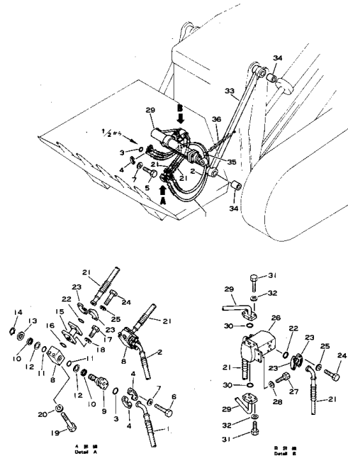
Fig. 125 HYDRAULIC PIPING (DBB050-1A Serial No. 1001~ (DBB057-1A Serial No. 1001~(9000))
