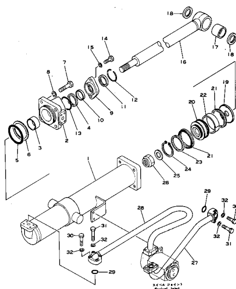
Fig. 111 CYLINDER (シリンダ) (DBB050-1A Serial No. 1001- ) (DBB057-1A Serial No. 1001- (9000))
