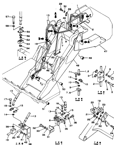
Fig. 121 HYDRAULIC PIPING (1/2) (DBB050-1A Serial No. 1001~) (DBB057-1A Serial No. 1001~(9000))
