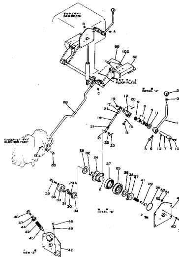
Fig-103 ACCELERATOR LINKAGE (1/2)
