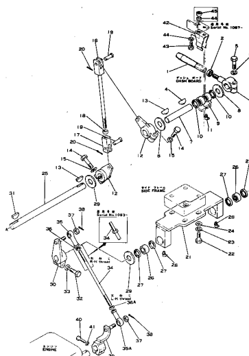
Fig.102 COMPRESSION RELEASE LINKAGE
