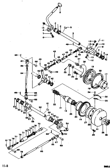
Fig.1107 ACCELERATOR LEVER (Serial No. 10001~ )
