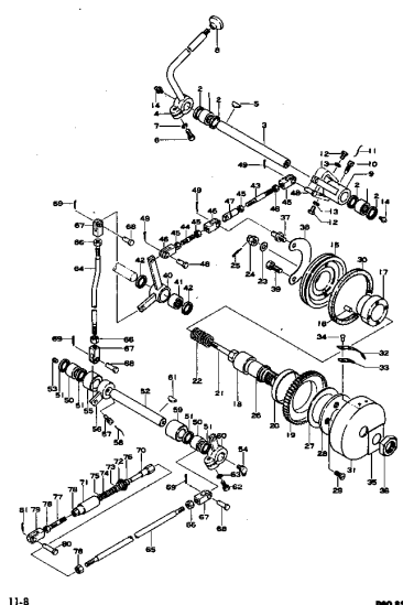
Fig.1107 ACCELERATOR LEVER (Serial No. 1001~ )
