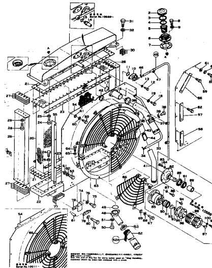
Fig. 1123 RADIATOR (適用機種C10001~21016) (Serial No.710001~20336)
