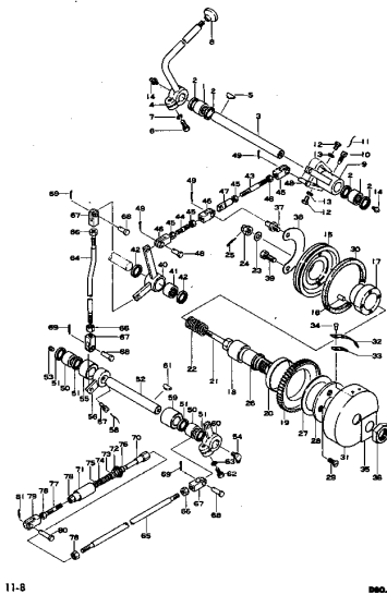
Fig.1107 ACCELERATOR LEVER (Serial No. 10001~ )
