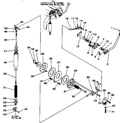
Fig. 104A FUEL CONTROL LEVER (適用号機 Serial No. 5022~)
