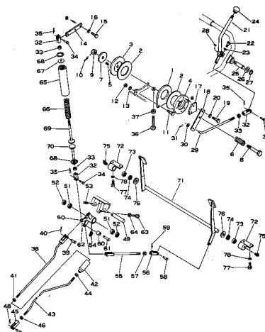
Fig. 1125 FUEL CONTROL LEVER AND DECELERATOR PEDAL (D65S Serial No. 20006-)
