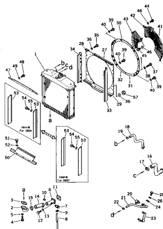
Fig. 134 RADIATOR PIPING AND COVER (D65A Serial No. 40001~ / D65P Serial No. 40001~40026)
