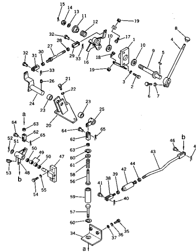
Fig. 122 FUEL CONTROL LEVER
