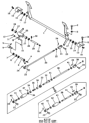
Fig. 1122A DECELERATOR PEDAL (D65A Serial No. 20024~) (D65P Serial No. 30001~)
