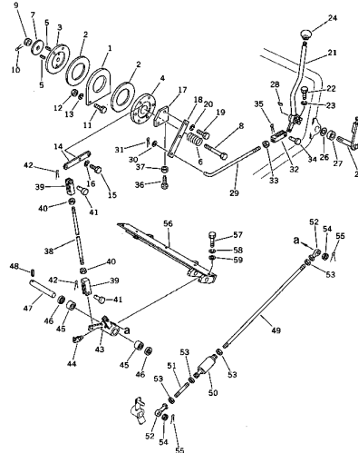
Fig. 121 FUEL CONTROL LEVER (D60S Serial No. 45001--)
