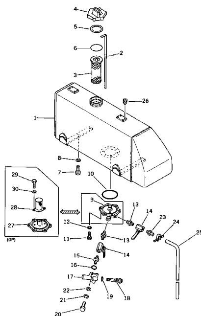
Fig. 141 FUEL TANK
