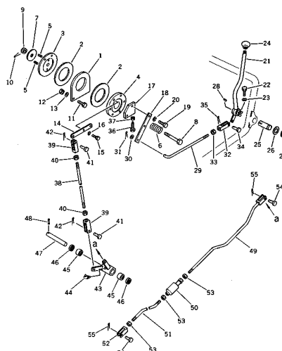
Fig. 121 FUEL CONTROL LEVER (D60S Serial No. 40001~)
