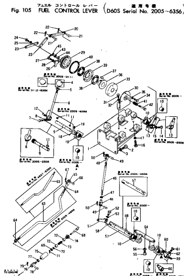
Fig. 105 FUEL CONTROL LEVER (D60S Serial No. 2005~6356)
