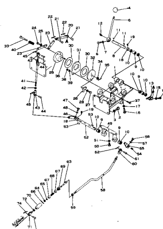
Fig. 105A FUEL CONTROL LEVER (D60S Serial No. 6357~)
