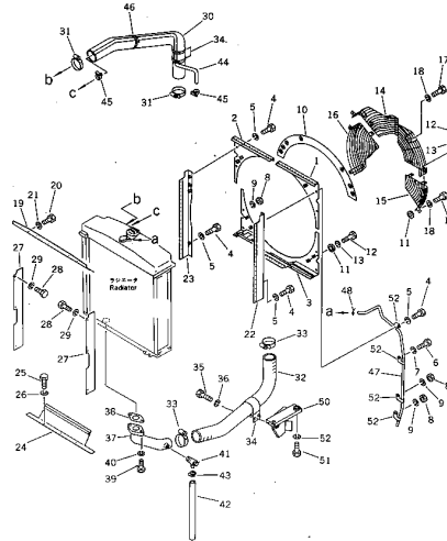
FIG. 134 RADIATOR PIPING AND COVER
