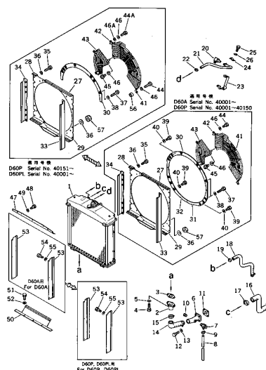
Fig. 133 RADIATOR PIPING AND COVER
