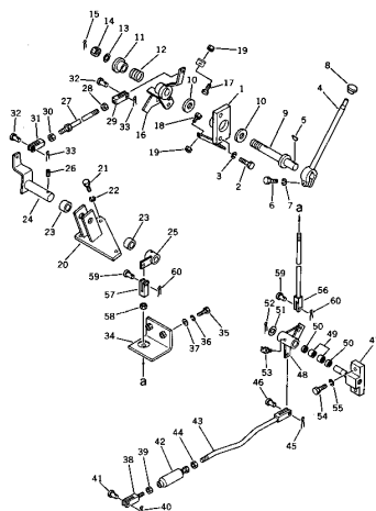
Fig. 121 FUEL CONTROL LEVER
