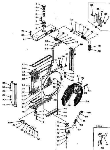
Fig. 122 RADIATOR (D60A, P Serial No. 2009-5709)
