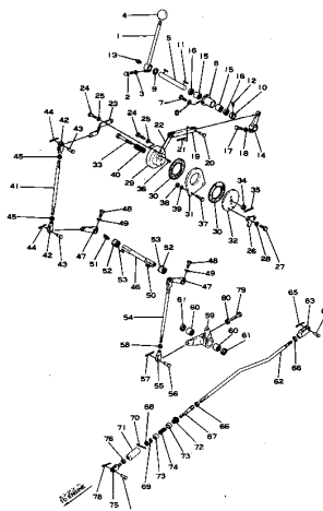
Fig. 104A FUEL CONTROL LEVER (D60A, P Serial No. 6357-)
