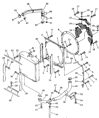
FIG. 133 RADIATOR PIPING AND COVER
