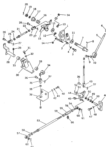
FIG. 121 FUEL CONTROL LEVER
