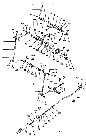
Fig. 104A 030050 FUEL CONTROL LEVER (D60A, P Serial No. 6357-)
