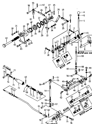
Fig. 104 FUEL CONTROL LEVER (D60A,P Serial No. 2009~6356)
