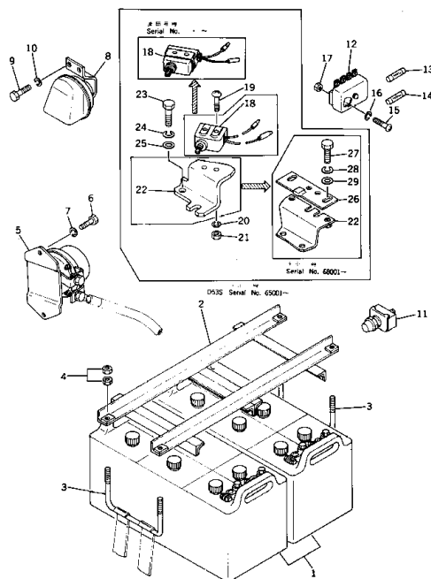
Fig. 151 BATTERY AND SWITCH
