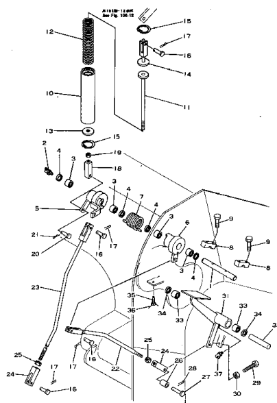
Fig. 107 FUEL CONTROL LEVER (2/2) (適用機種 Serial No. D53S 60001~)
