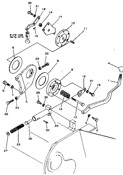
Fig. 106 FUEL CONTROL LEVER (1/2) (適用機種 Serial No. D53S 60001~)
