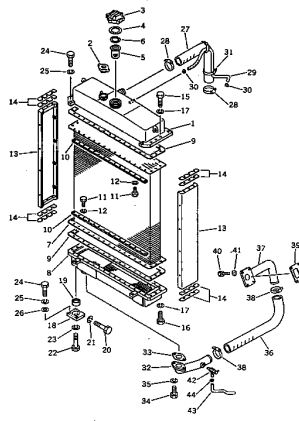
Fig. 2801 RADIATOR AND PIPING (Noise Suppression for EC) (D33A Serial No. 80001~) (D33P Serial No. 80943~)
