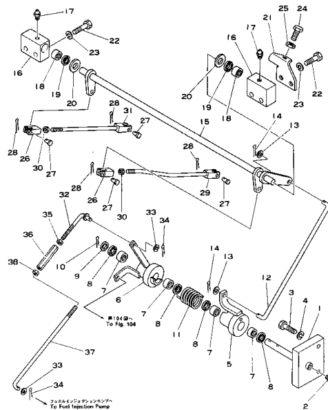
Fig. 105 FUEL CONTROL LEVER (2/2) (適用号機 (Serial No. D53A 60001~))
