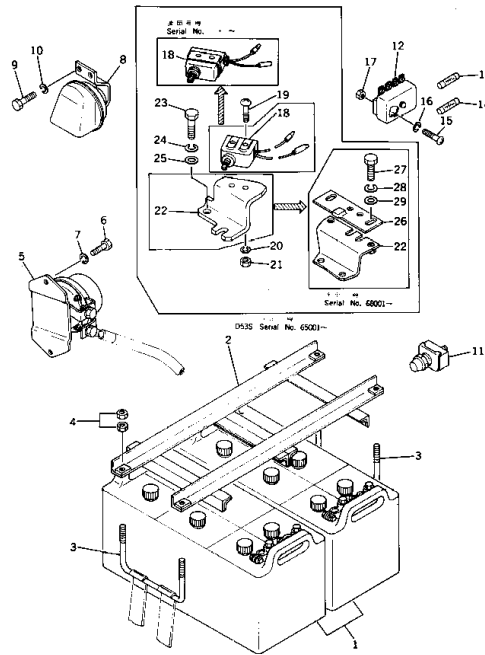
Fig. 151 BATTERY AND SWITCH
