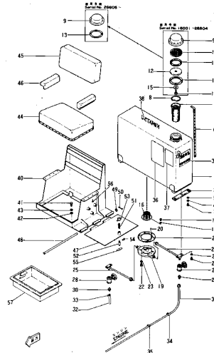
Fig. 112A FUEL TANK AND OPERATION'S SEAT (適用号機 D50S 16001~35000)
