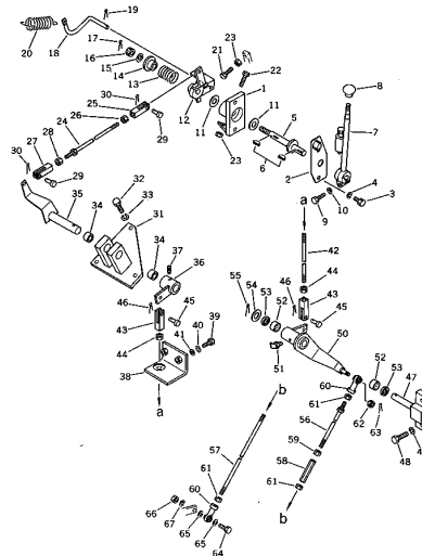
Fig. 121 FUEL CONTROL LEVER
