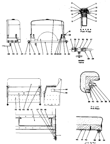
Fig. 111 FUEL TANK AND OPERATOR'S SEAT (Serial No. D50A.P 711~5860)
