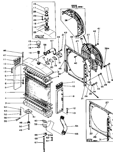
Fig. 1121 RADIATOR (Serial No. 35002~) (1/2)
