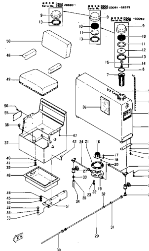
Fig. 111B FUEL TANK AND OPERATOR'S SEAT (Serial No. D50A, P 16001~35000)
