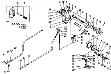
Fig. 103B FUEL CONTROL LEVER (適用号機 (Serial No. D50A, P 10901~35000) (Serial No. D50S, 3771~35000))
