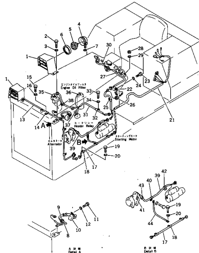
FIG. 1161 ELECTRICAL SYSTEM (1/2)
