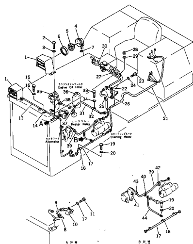
FIG. 1161 ELECTRICAL SYSTEM (1/2)
